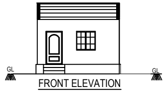
FRONT ELEVATION
