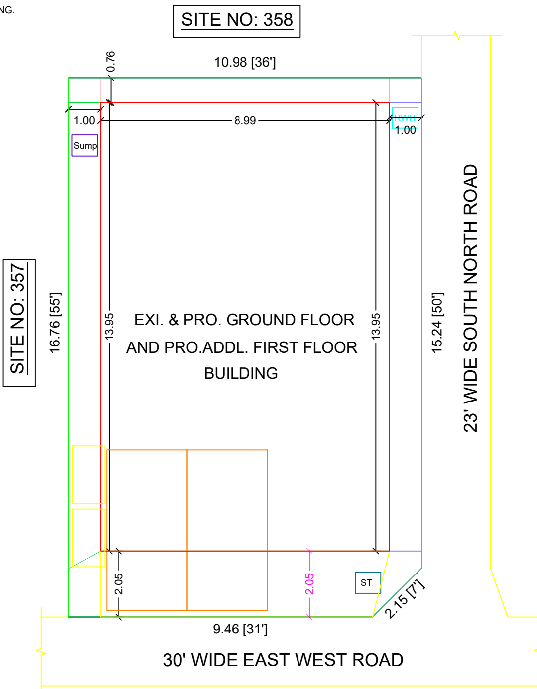
SITE PLAN (SCALE 1" EQ 8'-0")
