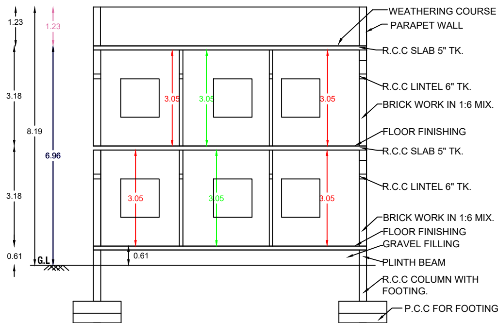
SECTION ON "AA" (SCALE 1" EQ 8'-0")
