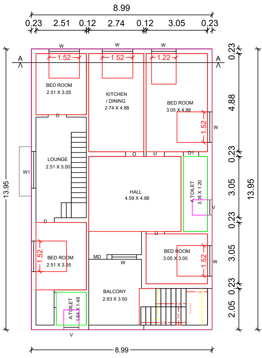
PRO.ADDITIONAL FIRST FLOOR PLAN (SCALE 1" EQ 8'-0")
