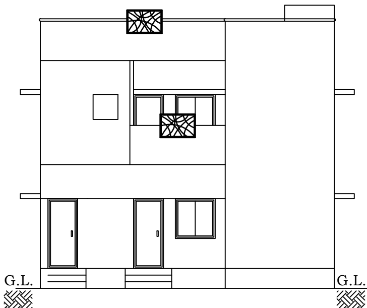
FRONT ELEVATION (SCALE 1" EQ 8'-0")
