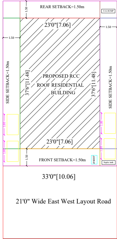
SITE PLAN
