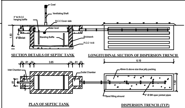
DETAILS OF SEPTIC TANK - 250 GALLONS & DISPERSION TRENCH
