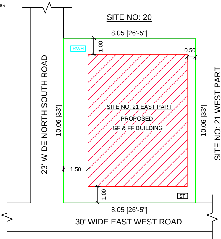
SITE PLAN
