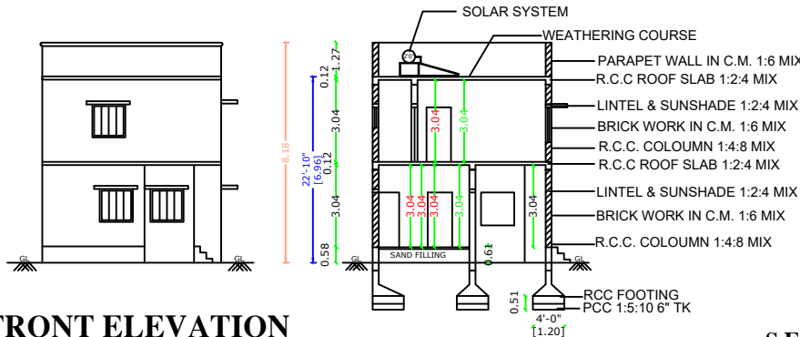
CROSS SECTION ON AA
