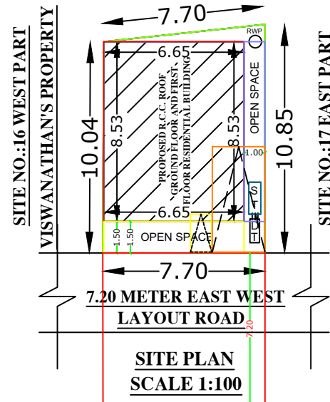
S.F.NO.:363/1B LAND LAYOUT AREA
