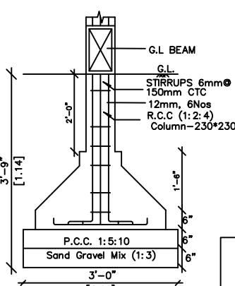
R.C.C. COLUMN FOOTING DETAILS
