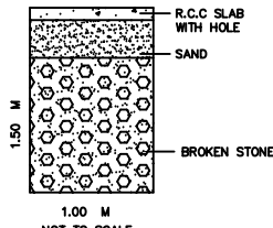
RAIN WATER HARVEST COLLECTION PIT.
