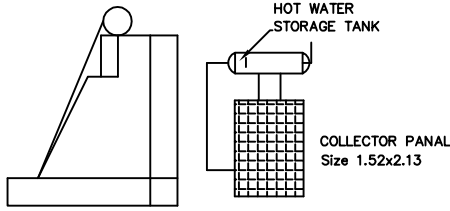
SIDE VIEW FRONT VIEW SOLAR WATER HEATER DETAILS
