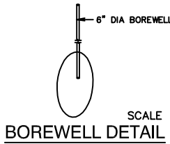
BOREWELL DETAIL
