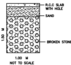
RAIN WATER HARVEST COLLECTION PIT.
