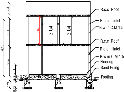
SECTION AB
