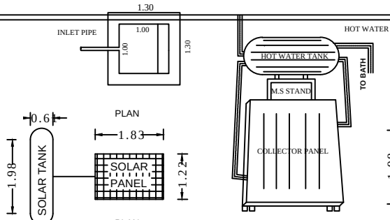
SOLAR WATER HEATER SYSTEM
