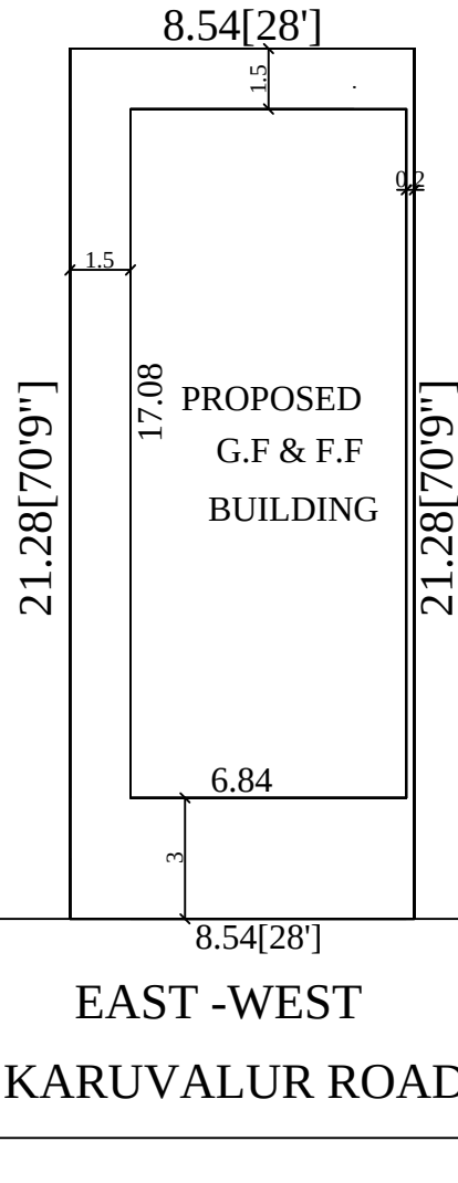
SITE PLAN
