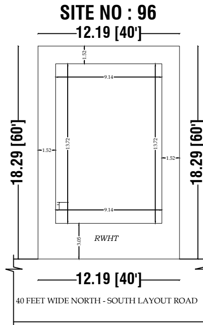
SITE PLAN
