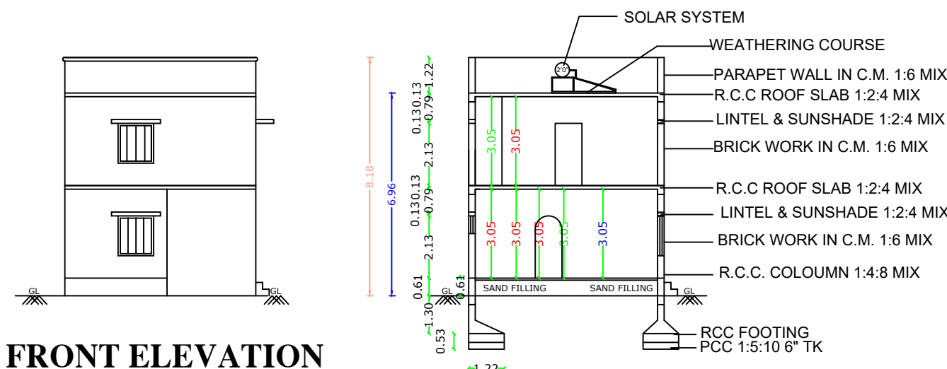
CROSS SECTION ON AA
