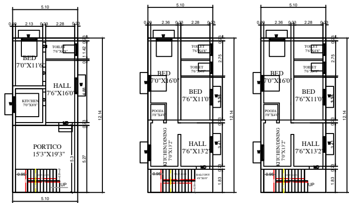
PROPOSED GROUND FLOOR PLAN PROPOSED FIRST FLOOR PLAN PROPOSED SECOND FLOOR PLAN
