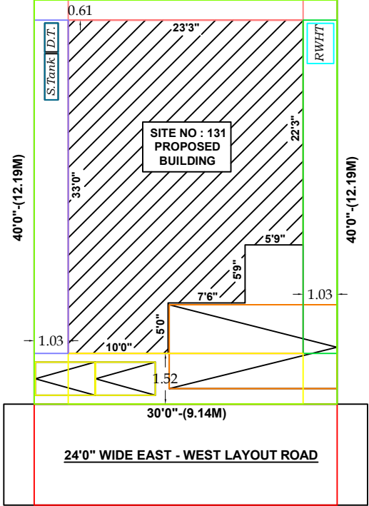
SITE PLAN
