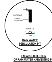
ENLARGED SECTION OF RAIN WATER HARVESTING PIT
