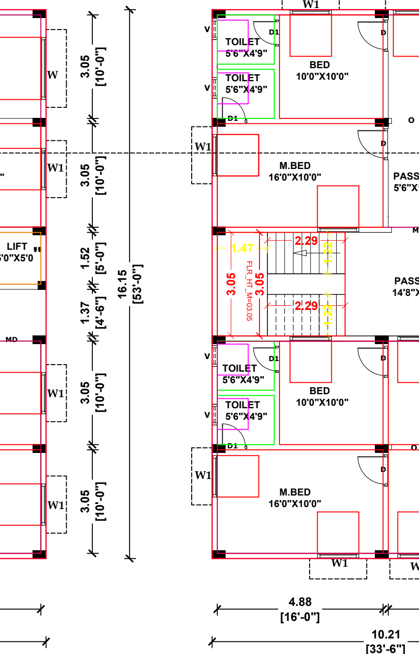
PROPOSED THIRD FLOOR PLAN
