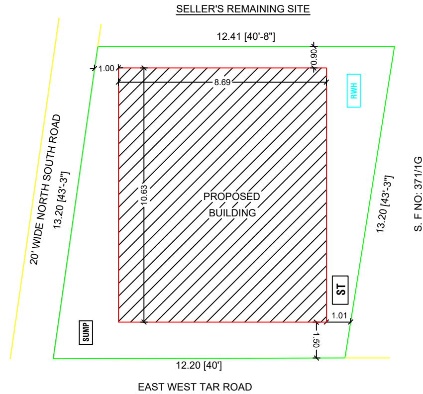
SITE PLAN
