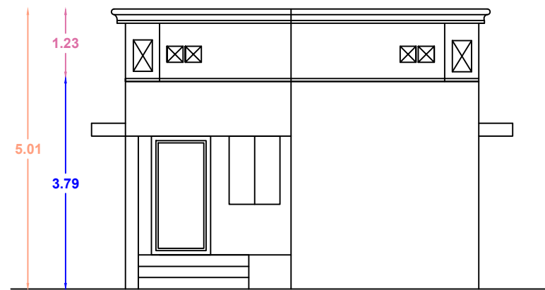
NORTH SIDE ELEVATION
