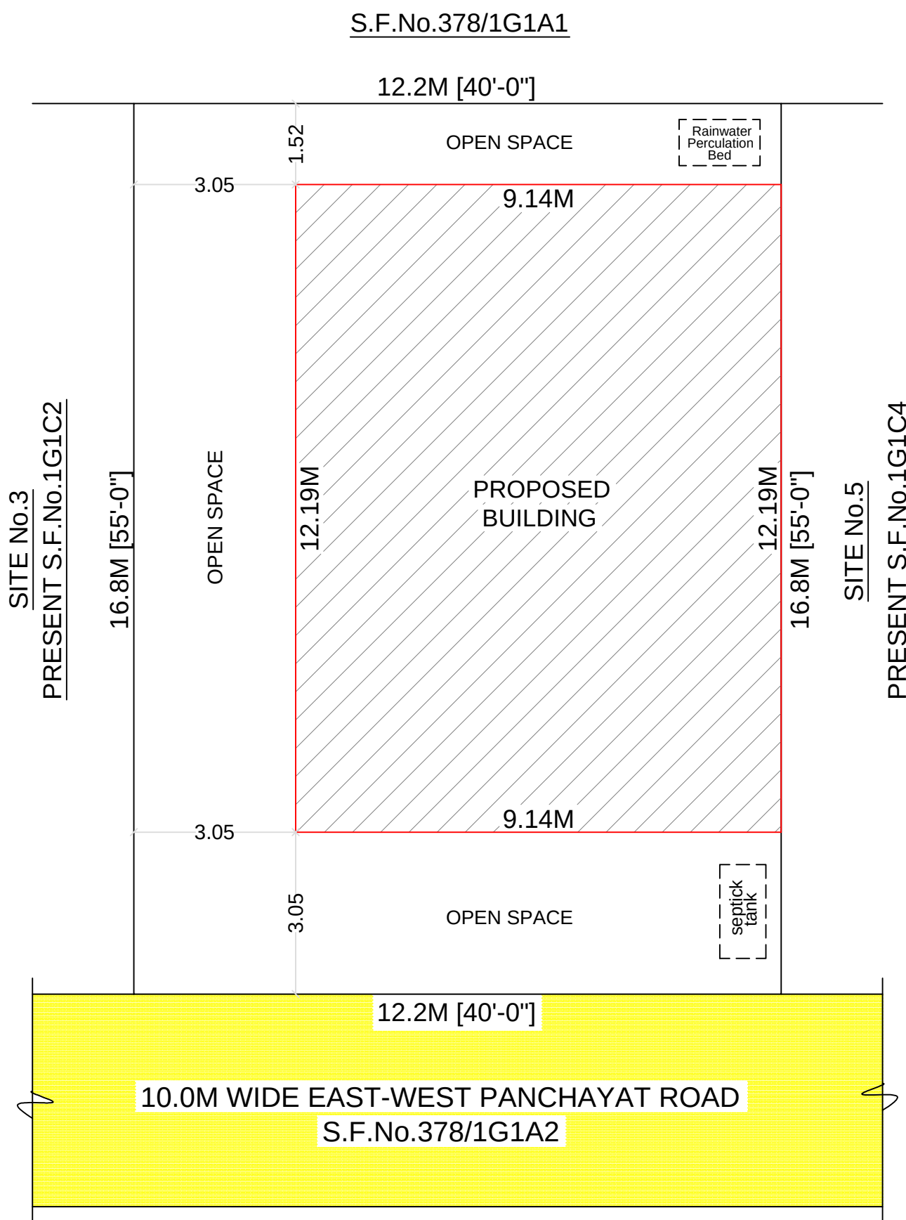
SITE PLAN
