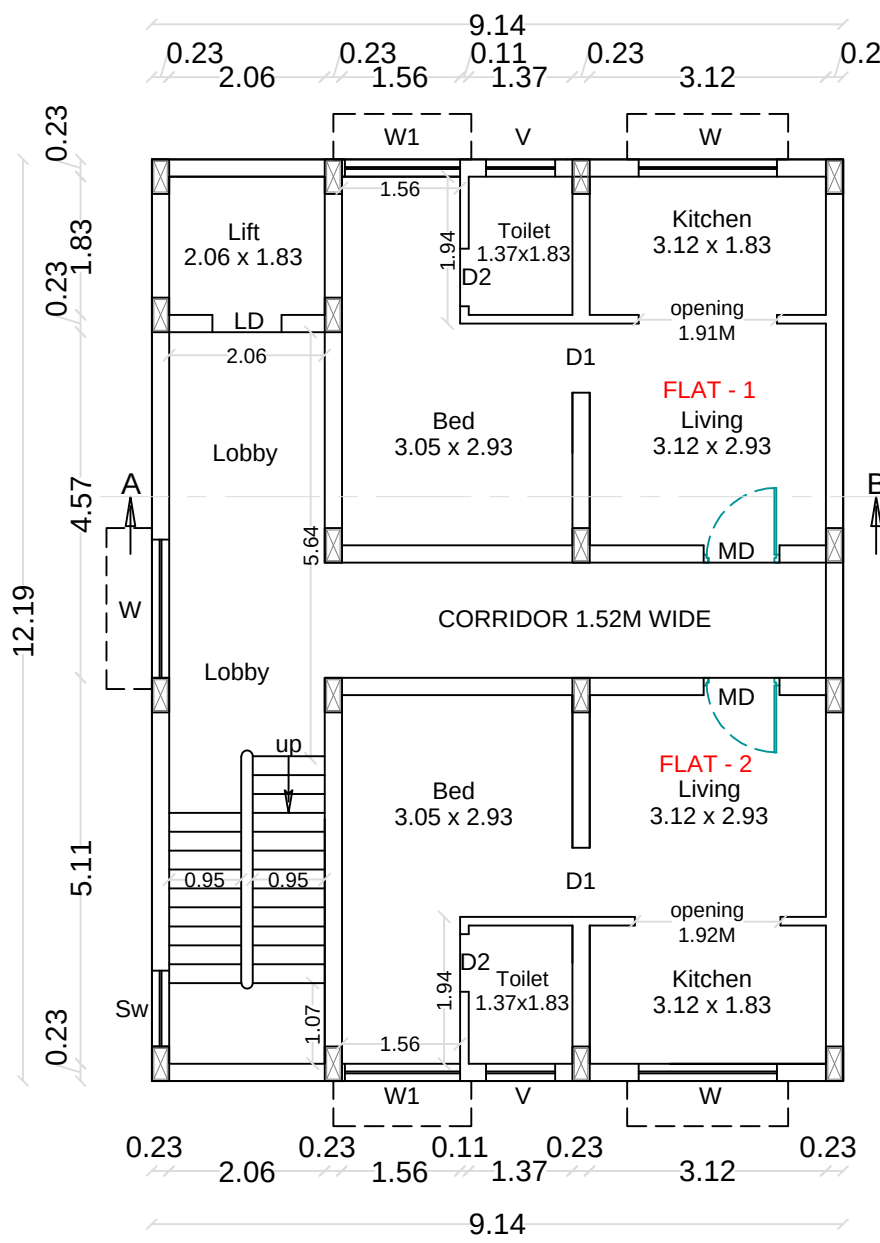
TYPICAL FLOOR PLAN (FIRST, SECOND AND THIRD FLOORS)
