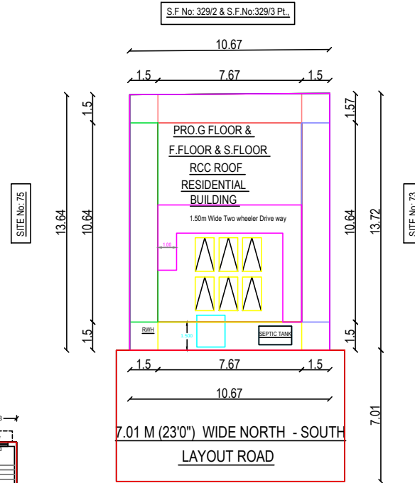
SITE PLAN
