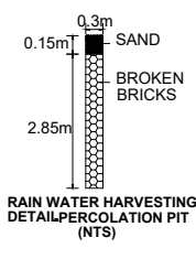
RAIN WATER HARVESTING DETAIL PERCOLATION PIT (NTS)
