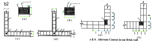
Figure - 2 Typical Details of Providing Vertical Steel Bars in Brick Masonry.
