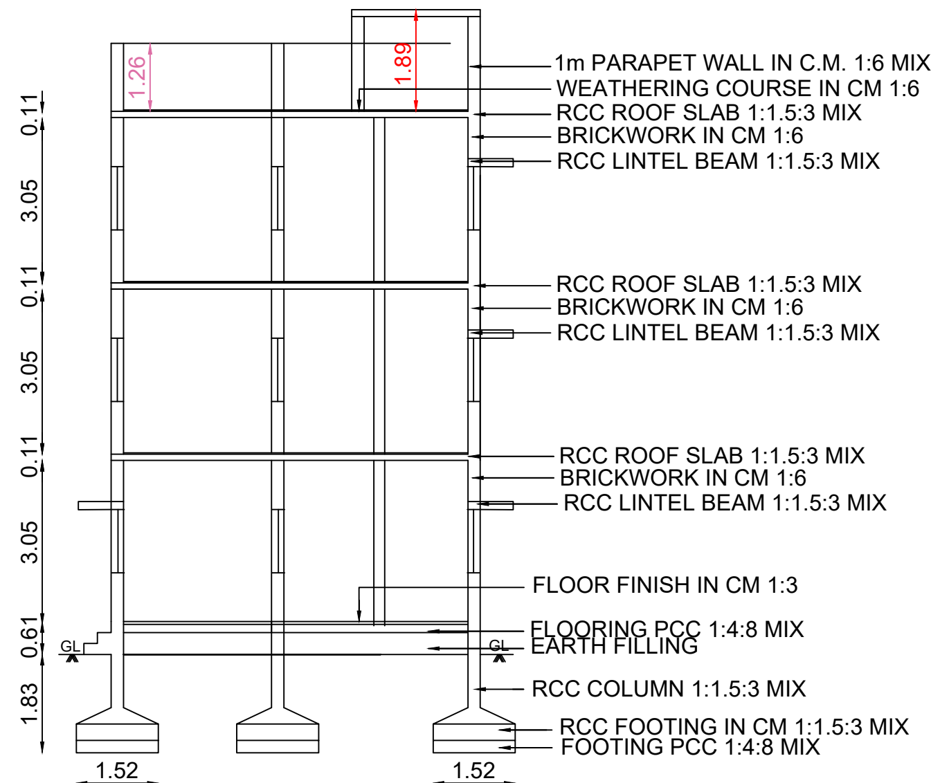
CROSS SECTION ON XY
