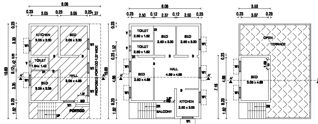
PROPOSED SECOND FLOOR PLAN
