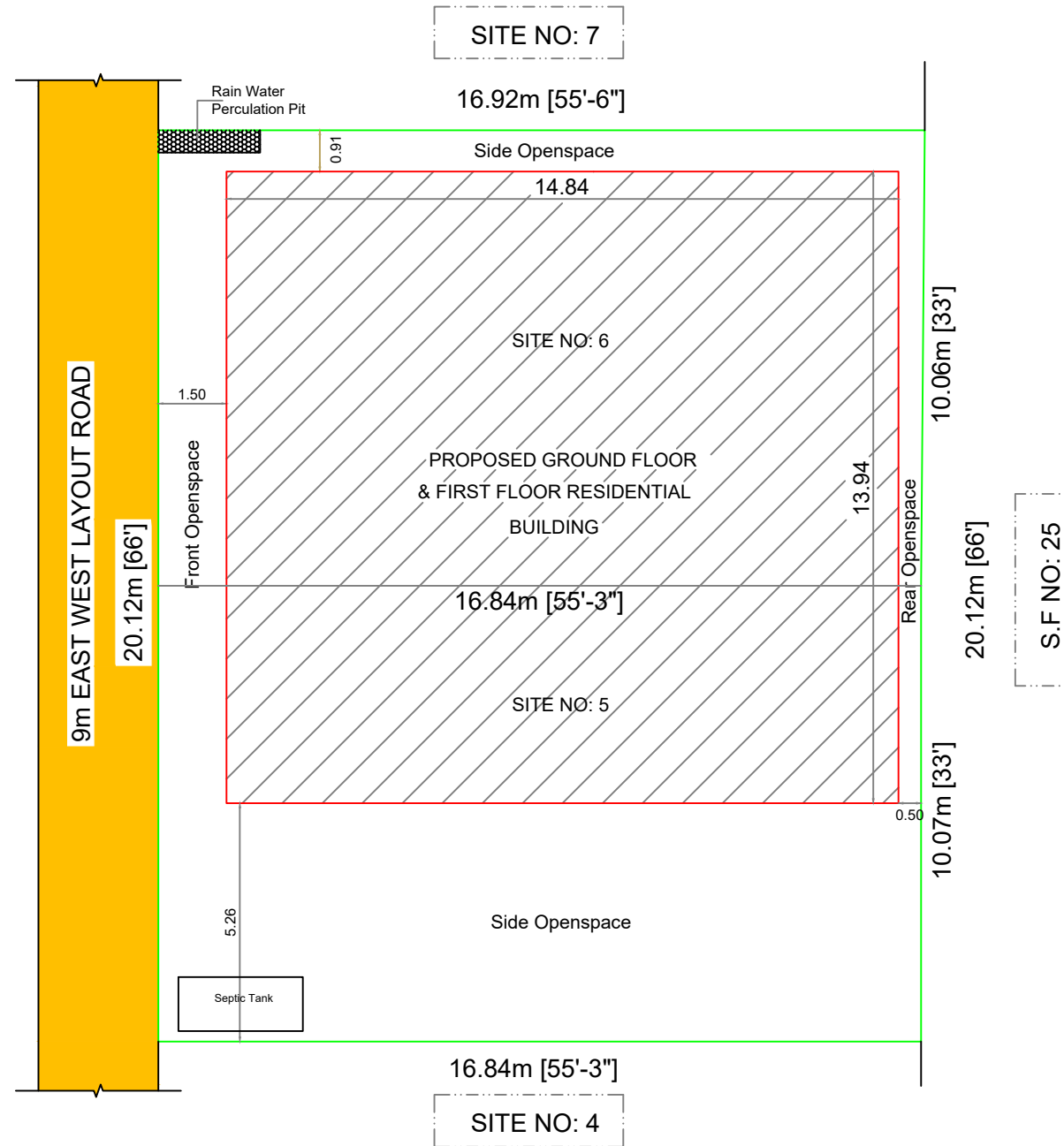
SITE PLAN
