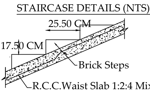
STAIRCASE DETAILS (NTS)
