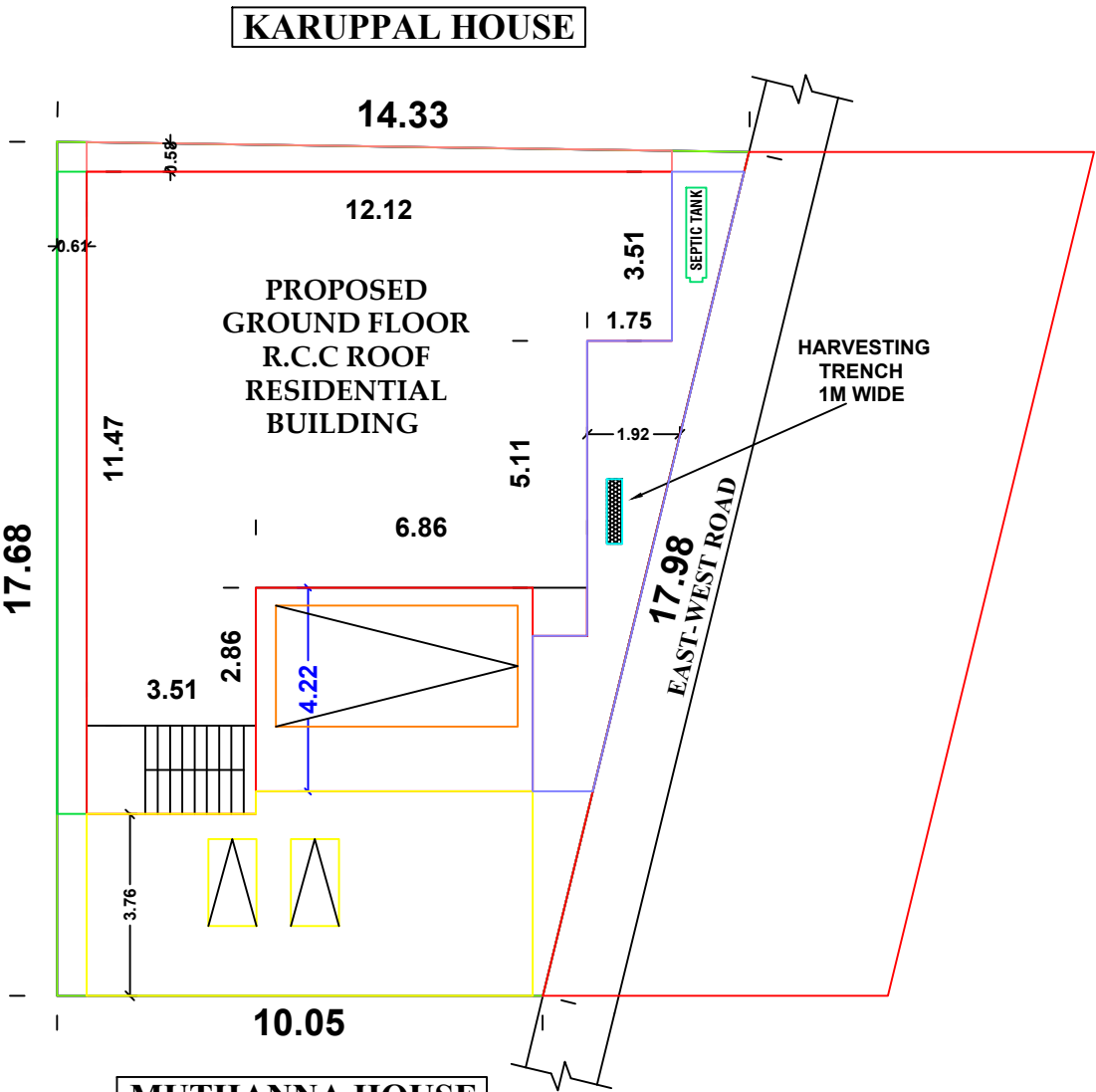
SITE PLAN
