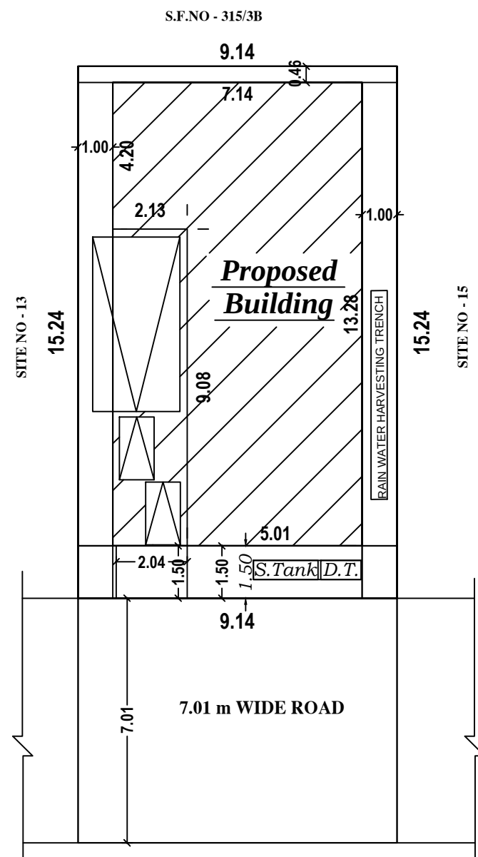
SITE PLAN
