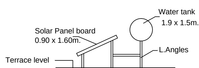
CROSS SECTION OF SOLAR WATER HEATING SYSTEM
