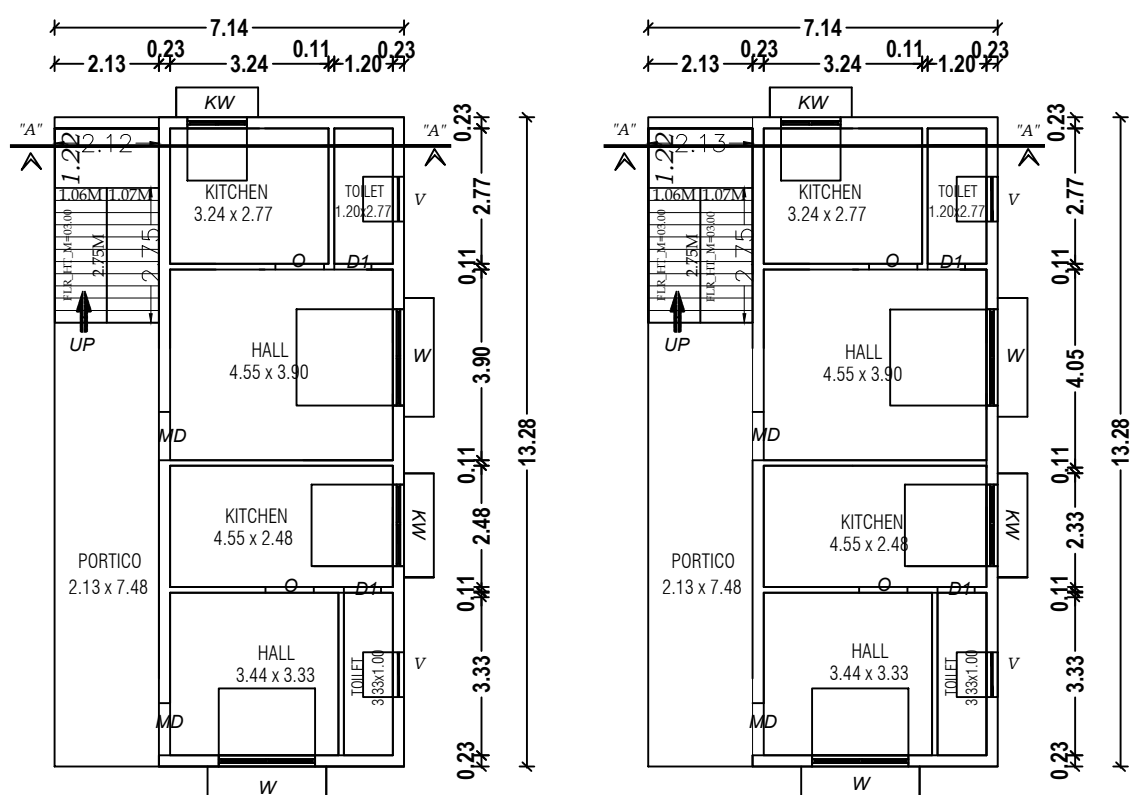
PRO.GROUND FLOOR PLAN PRO.FIRST FLOOR PLAN
