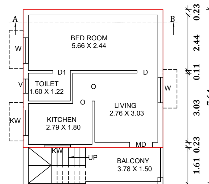
PROPOSED SECOND FLOOR
