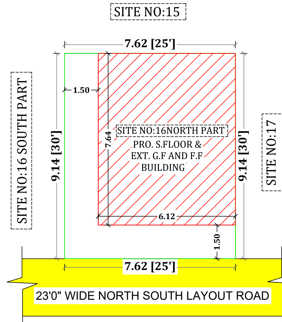
SITE PLAN
