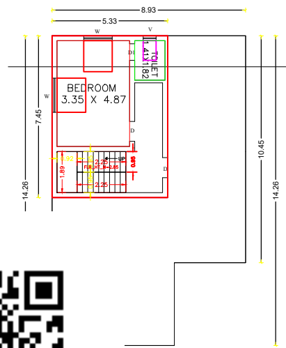
1 FLOOR PLAN
