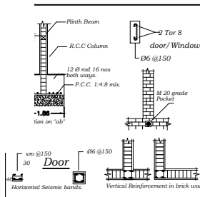
Horizontal Seismic bands Vertical Reinforcement in brick walls
