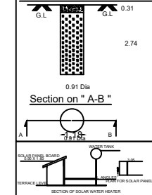
Detailed Plan of Rainwater Perculation and Collection Pit
