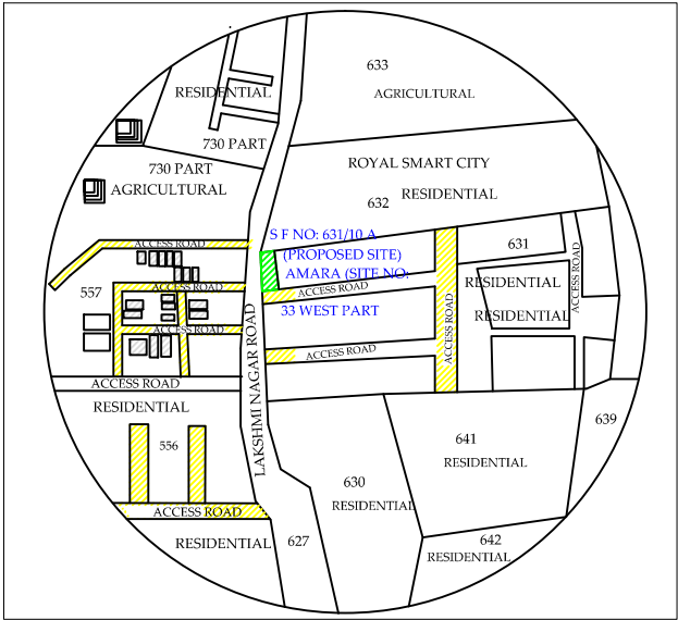
TOPO PLAN
