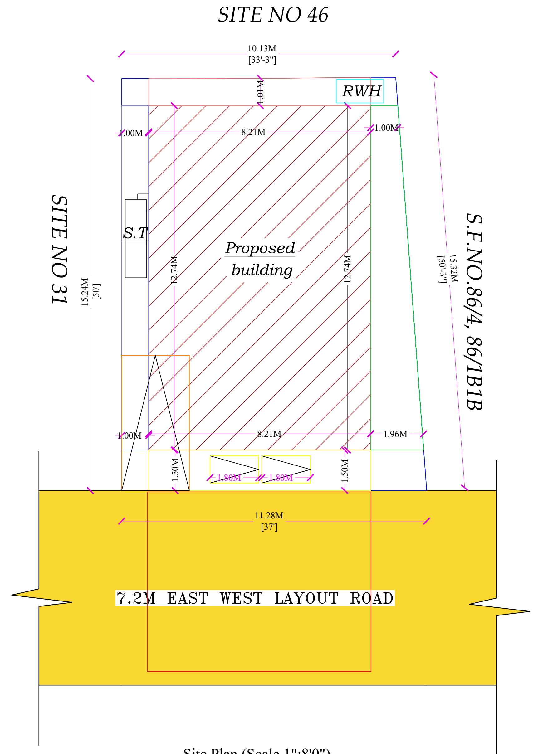
Site Plan (Scale 1"=8'0") SITE PLAN
