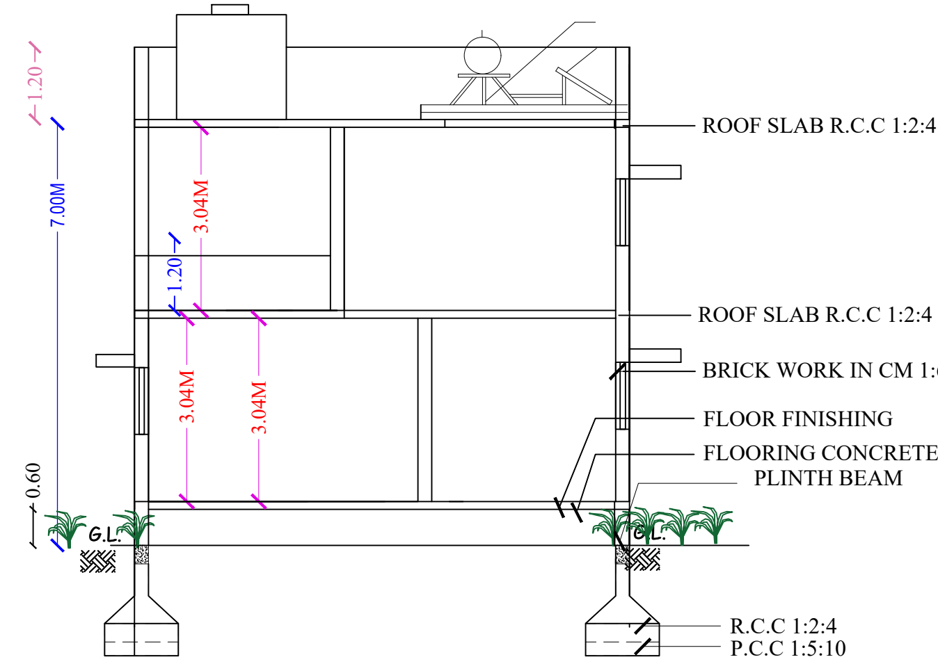
SECTION "A-A"
