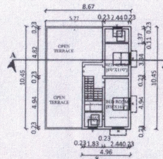
PRO. FIRST FLOOR
