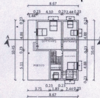
PRO. GROUND FLOOR
