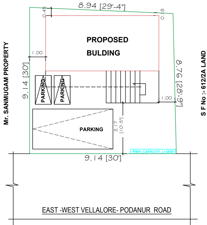
SITE PLAN
