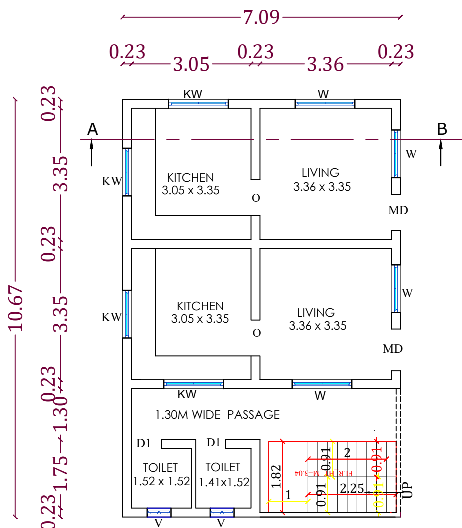
ADDL.& ALTERATION OF GROUND FLOOR PLAN
