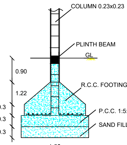
COLUMN DETAILS
