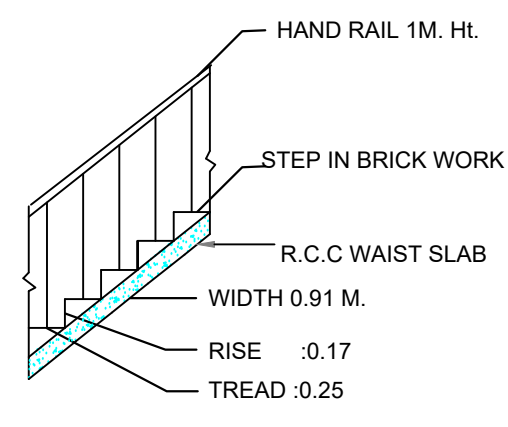
STAIR DETAIL
