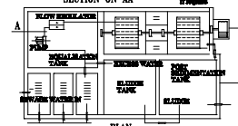
PLAN SEWAGE TREATMENT PLANT DETAILS (WASTE WATER WORKS REQUIRED)
