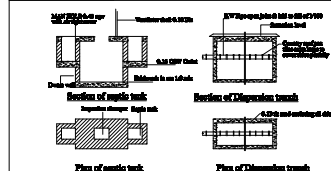
SEPTIC TANK
