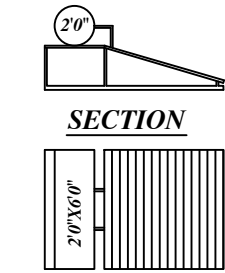
PLAN SOLAR WATER HEATER (NOT TO SCALE)
