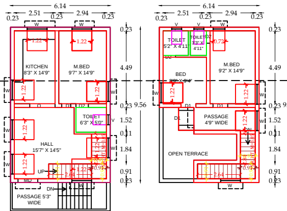
PRO. SECOND FLOOR PLAN
