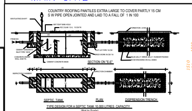
COUNTRY ROOFING PANTILES EXTRA LARGE TO COVER PARTLY 15 CM S W PIPE OPEN JOINTED AND LAID TO A FALL OF 1 IN 100
