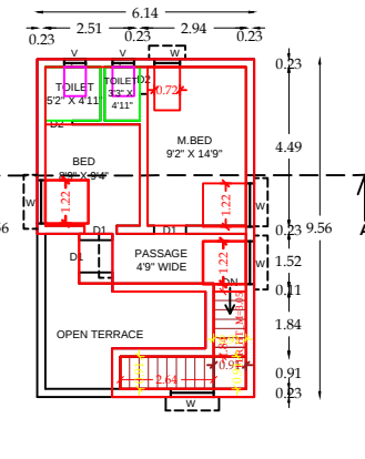
PRO. SECOND FLOOR PLAN
