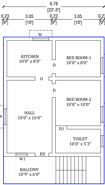
EXISITNG FIRST FLOOR PLAN
