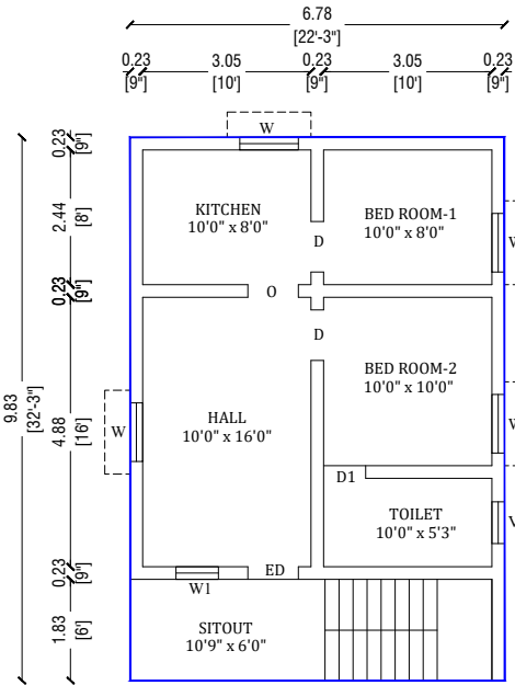
EXISITNG GROUND FLOOR PLAN
