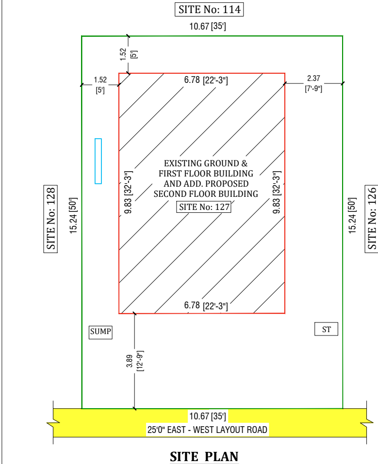
SITE PLAN
