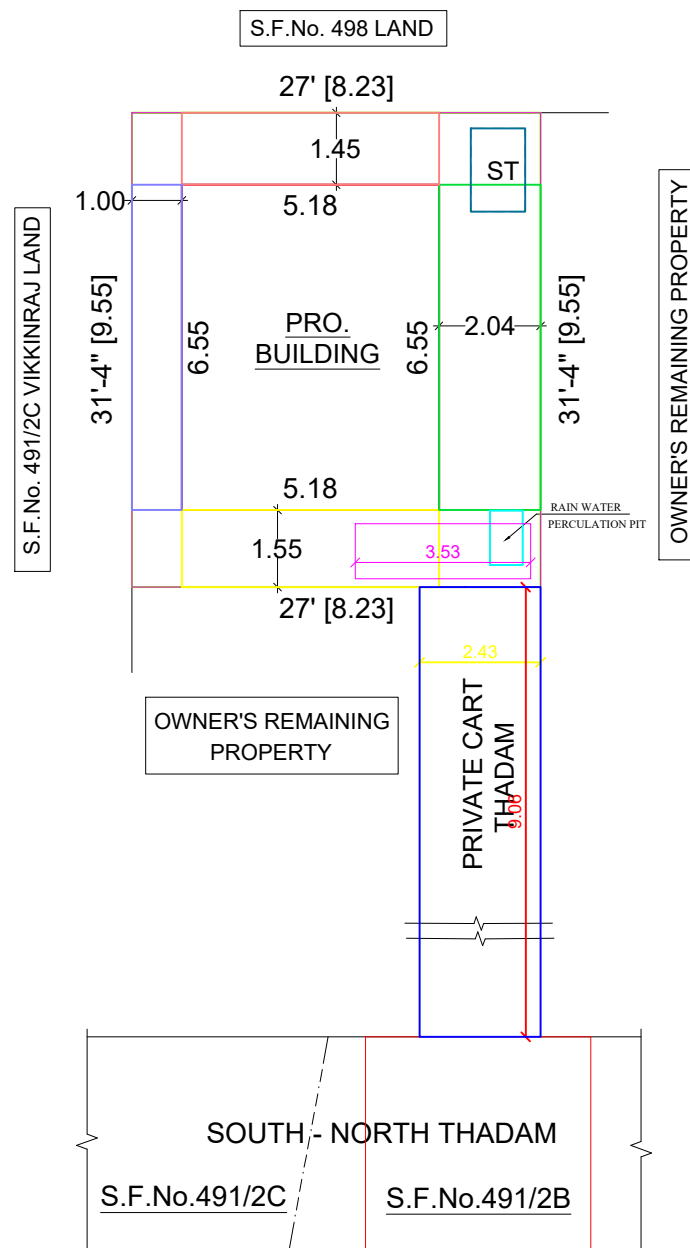
SITE PLAN
