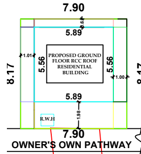
SITE PLAN
