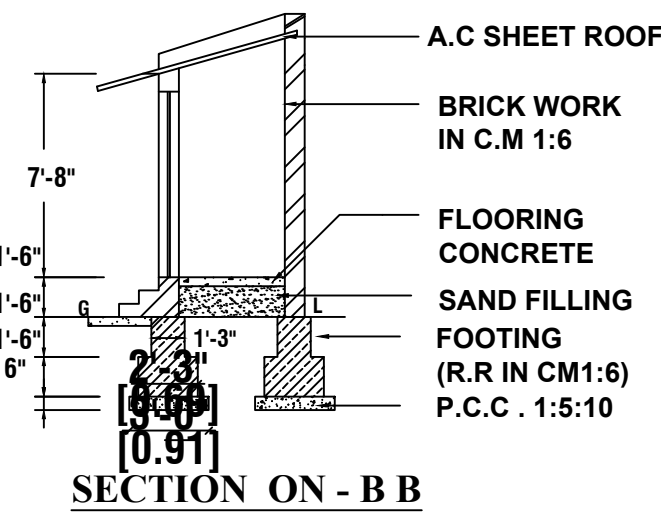
SECTION ON - B B
