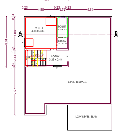
PROPOSED FIRST FLOOR PLAN
