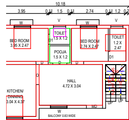
PROPOSED ADDITIONAL FIRST FLOOR BUILDING
