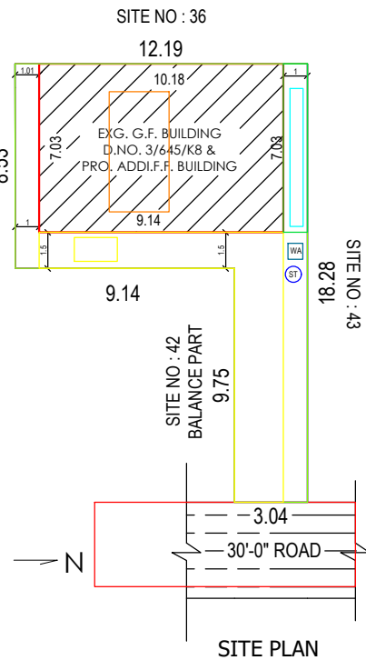
PROPOSED ADDITIONAL FIRST FLOOR BUILDING
