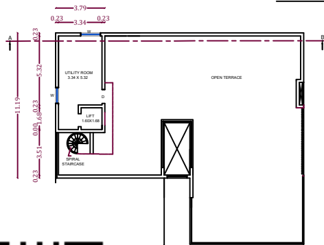
PROPOSED SECOND FLOOR PLAN
