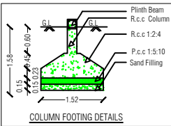
COLUMN FOOTING DETAILS
