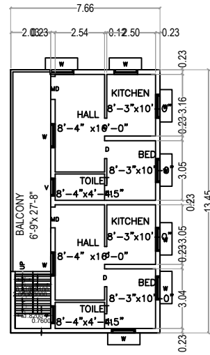
EXISTING FIRST FLOOR PLAN
