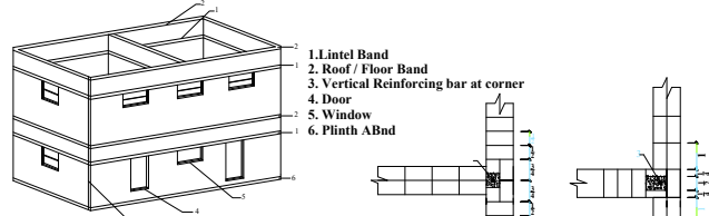
Figure - 1 : Essential Internal Elements in Building for Earthquake Safety.
