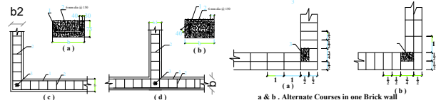
Figure - 2 : Reinforcement and Bending Details of Seismic Bands.
