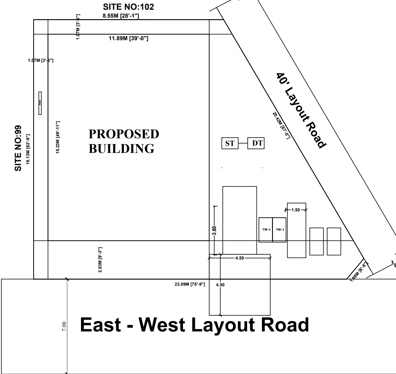
SITE PLAN
