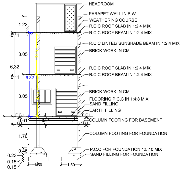
SECTION ON-AA
