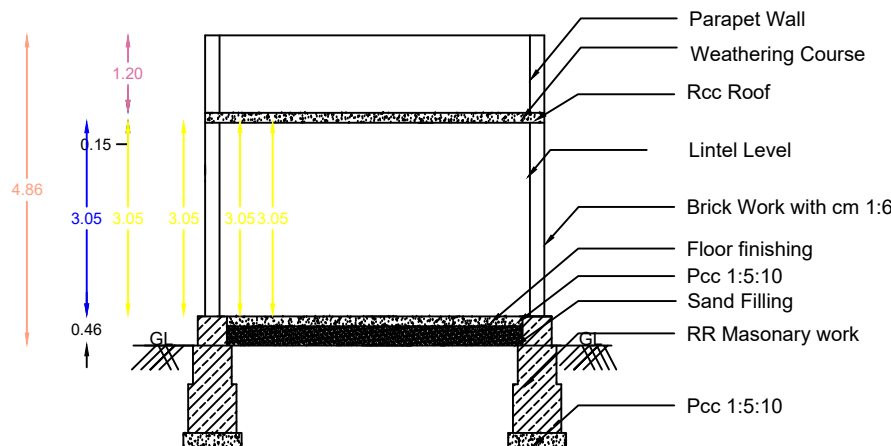
SECTION ON-"AB"
